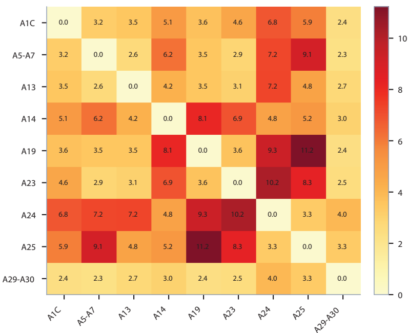
Astrocyte \omega across 9 brain regions
