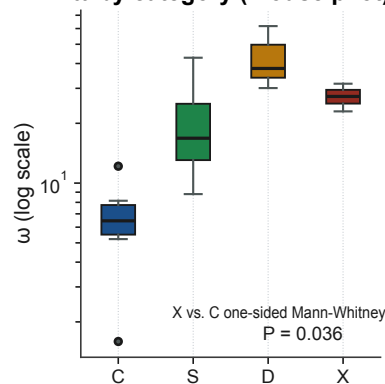
C \omega by category (mouse pilot)
