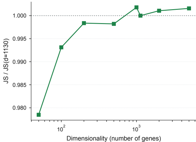
B. Dimensionality ratio (relative to HK gene set)
