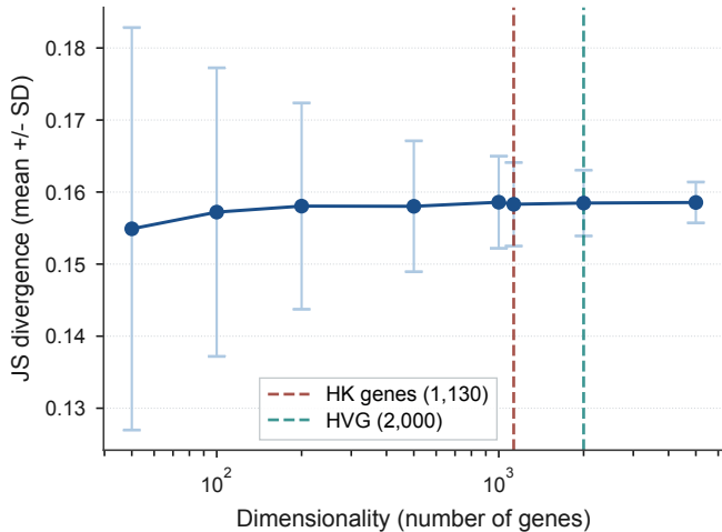
A. JS divergence vs dimensionality
