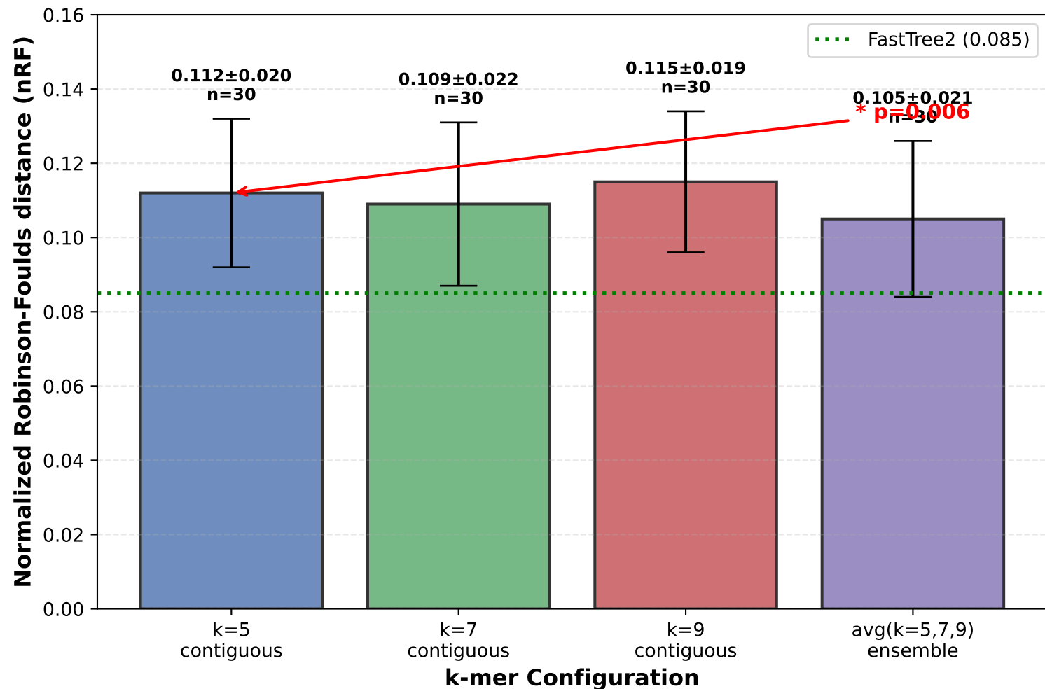
Figure 3. Multi-k Ensemble Improves Accuracy (n=200 Indel-Rich Data, 30 seeds)
