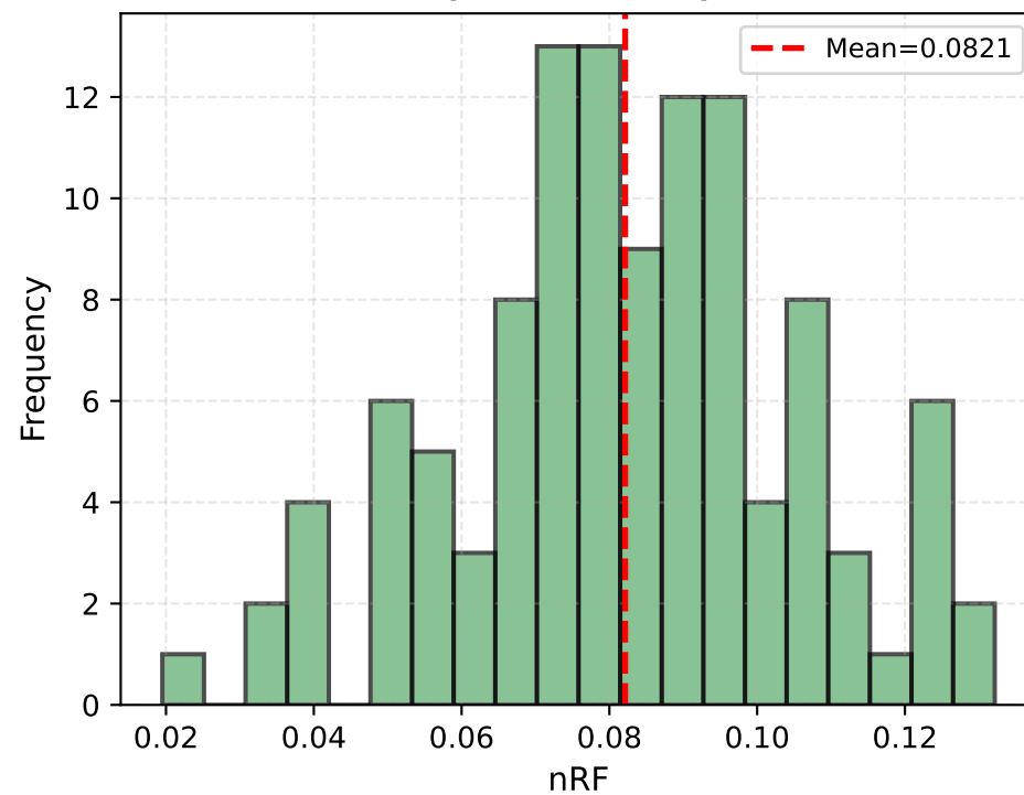
FastTree2 (n=200 indel)
