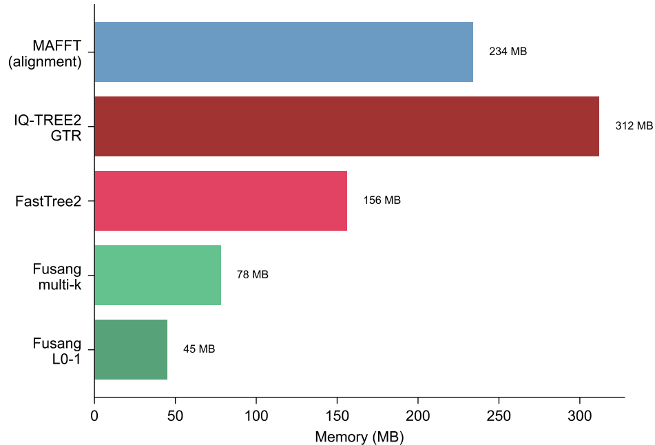
(B) Memory Usage (n=200)
