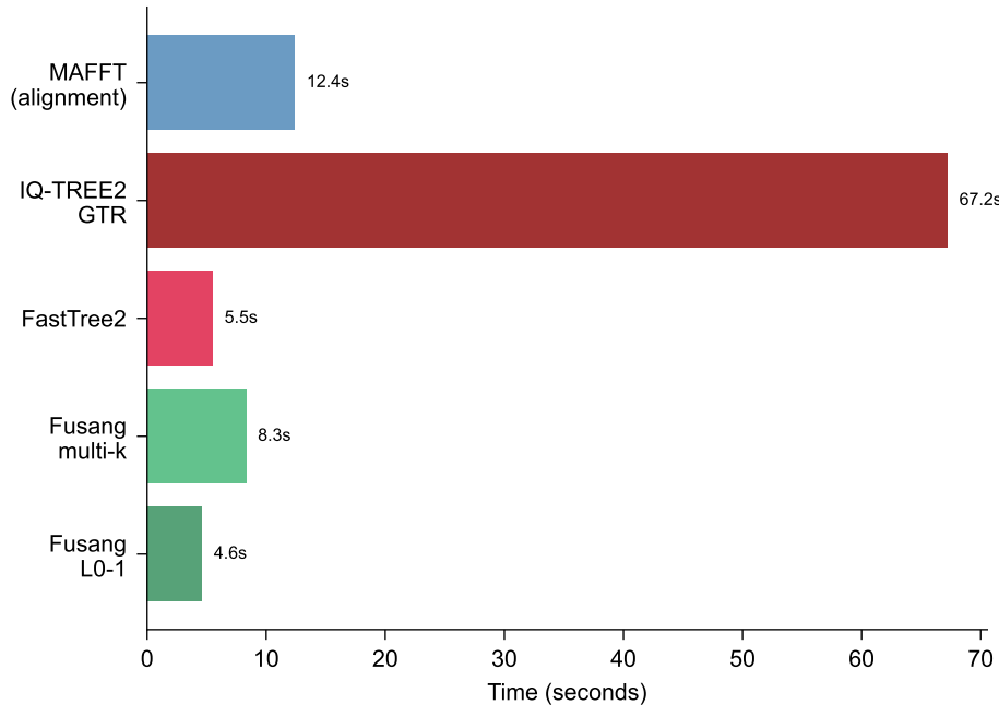
(A) Computational Time (n=200)
