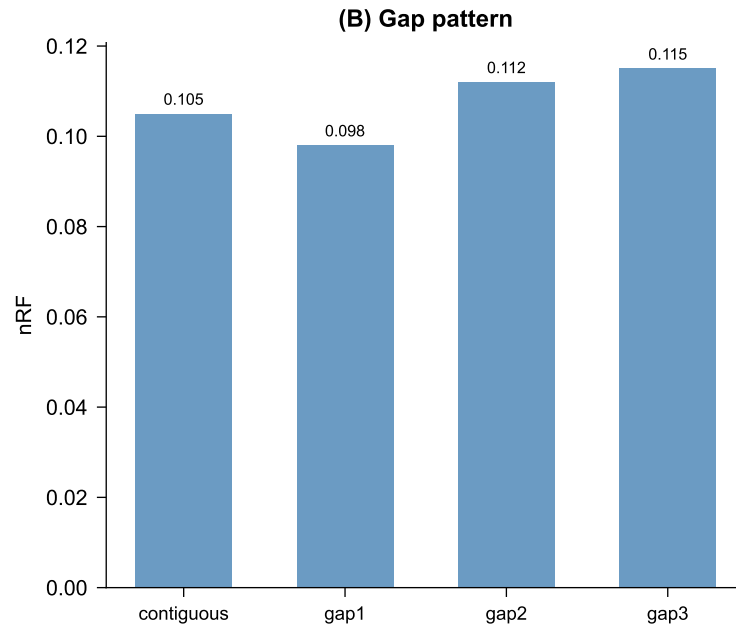
Supplementary Figure S6: k-mer Parameter Sensitivity
