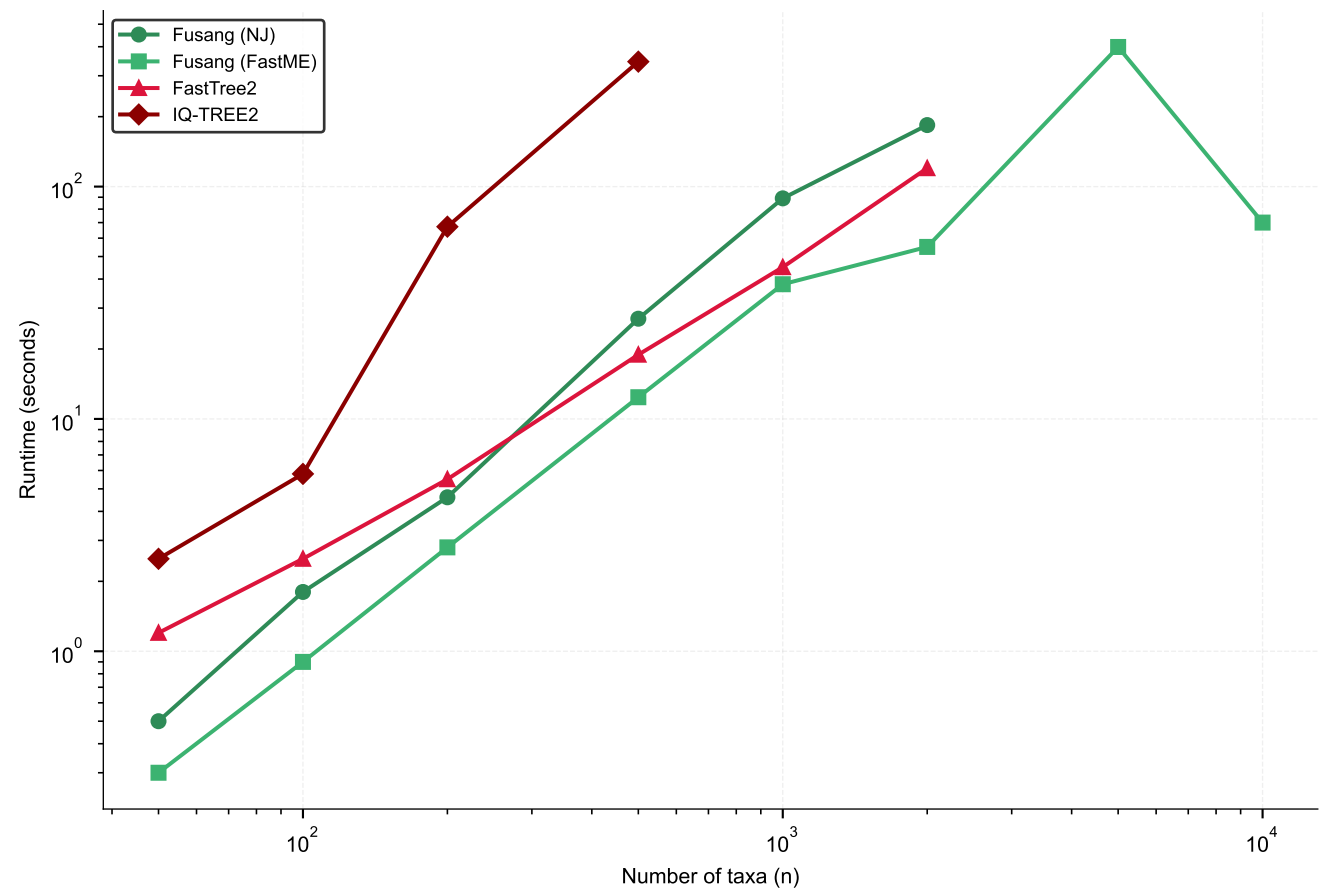
Supplementary Figure S8: Runtime Scaling by Taxa Number
