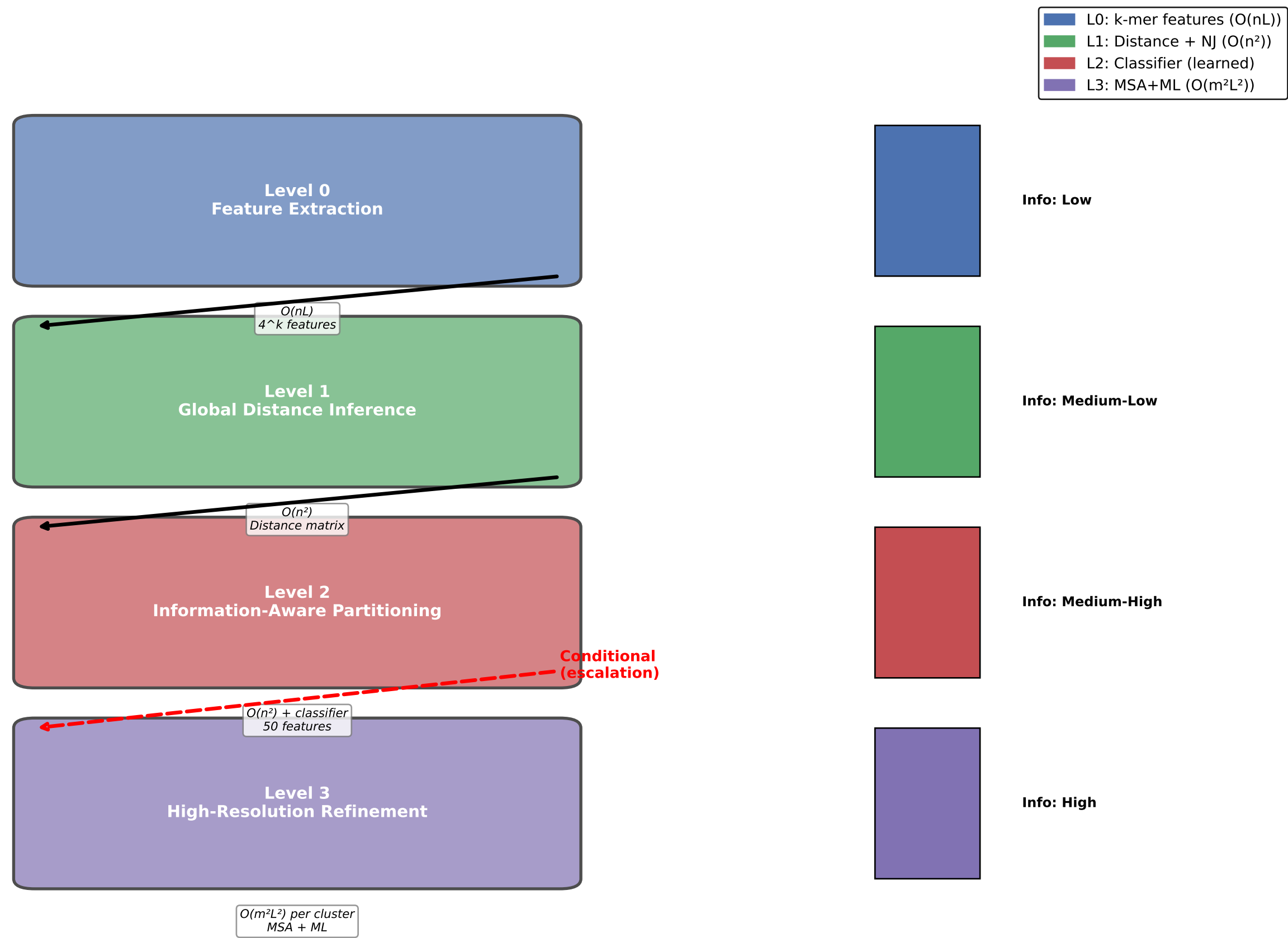
Figure 1. IMMI Framework Architecture (Information-Matched Multi-Level Inference)
