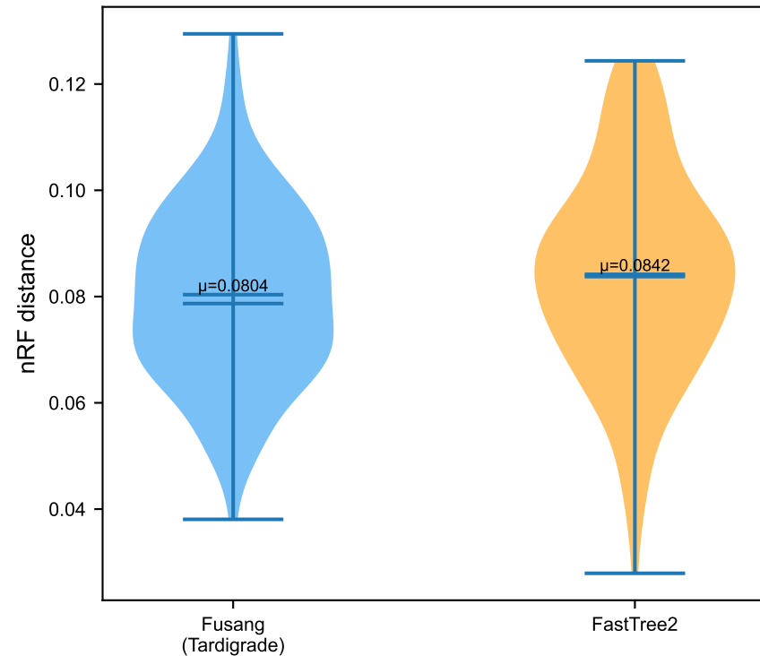
A. nRF Distribution ( n=200 , \text{indel}=0.02 , 130 seeds)
