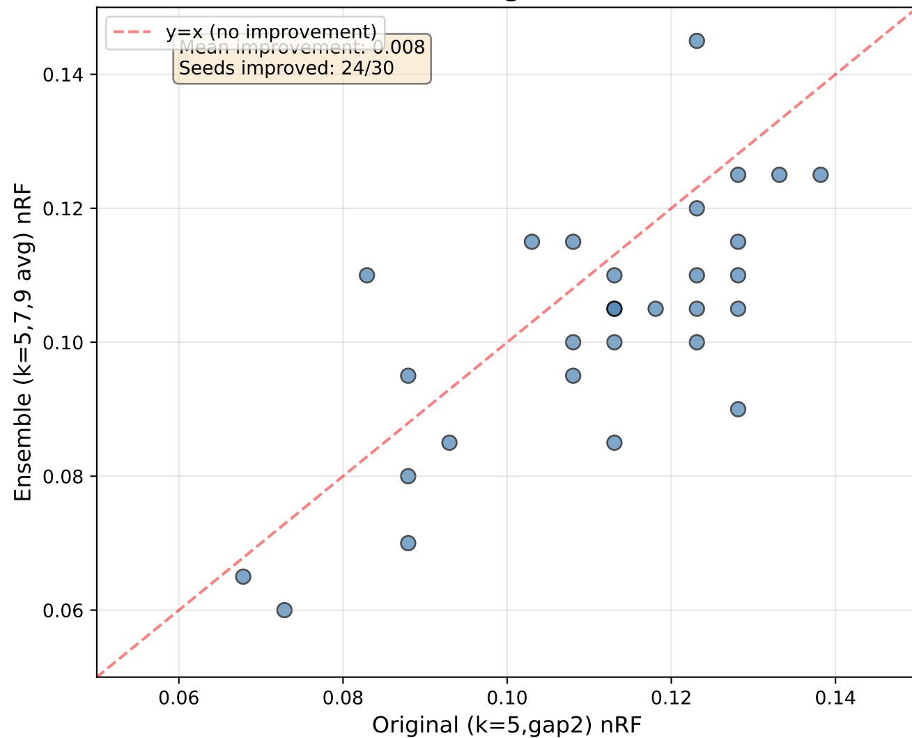
Per-seed nRF: Original vs Ensemble
