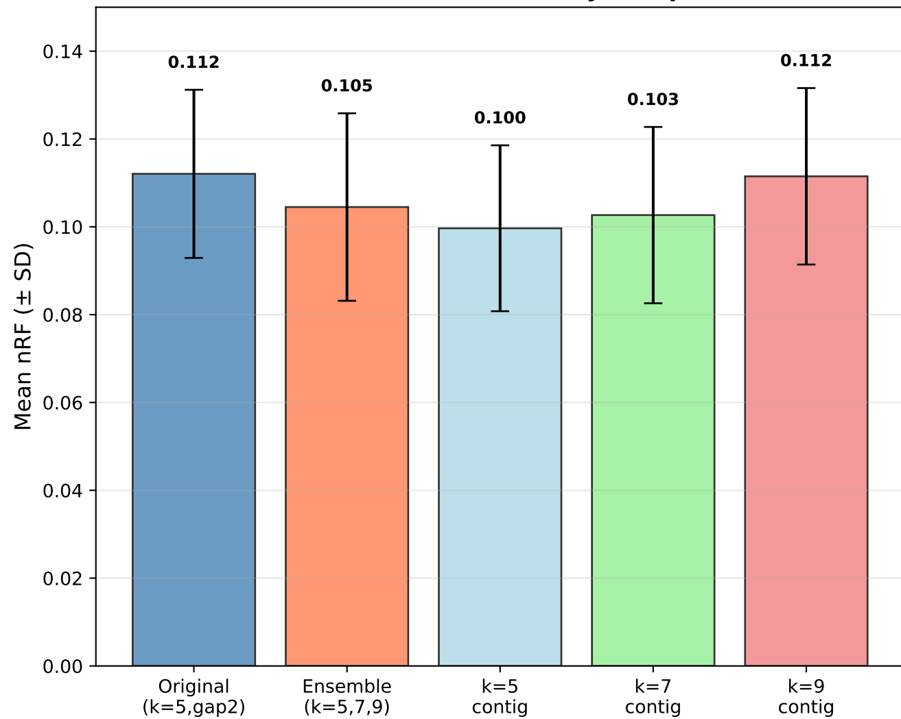
Multi-k Ensemble: Accuracy Comparison
