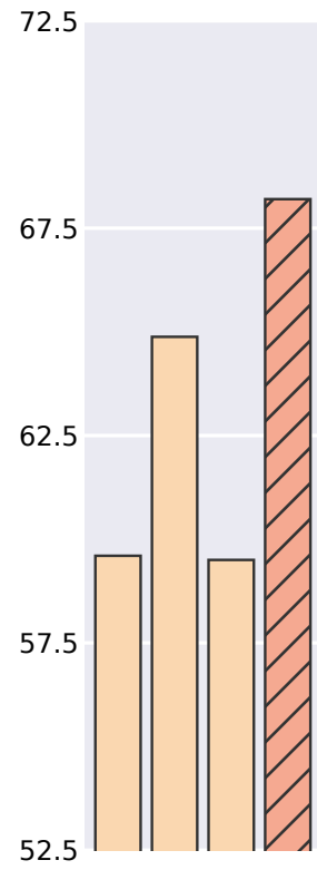
Math500
