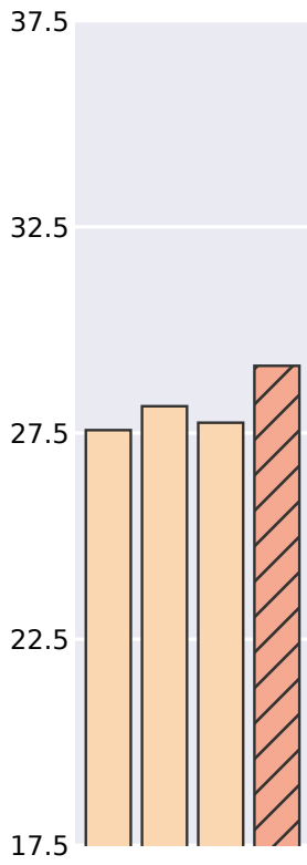
Olympiad Bench
