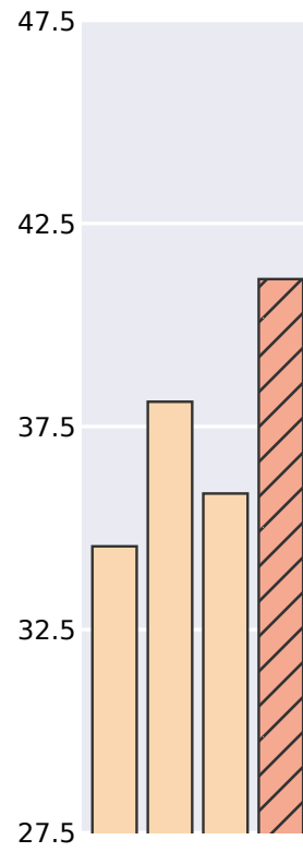
College Math
