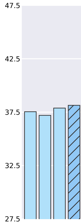
ARC challenge
