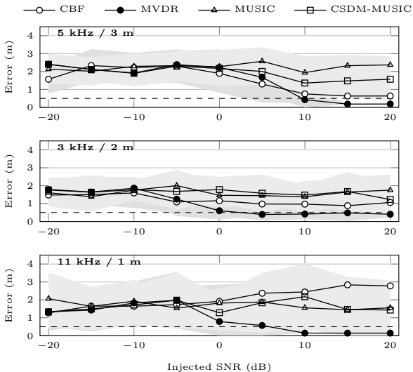
Figure 1: Mean localization error (over 20 projector events, \pm 1 std shaded) versus injected band-matched noise SNR for the four algorithms in three projector conditions (post-processing injection on the original 8-channel recordings; dashed: 0.5 m failure threshold).
