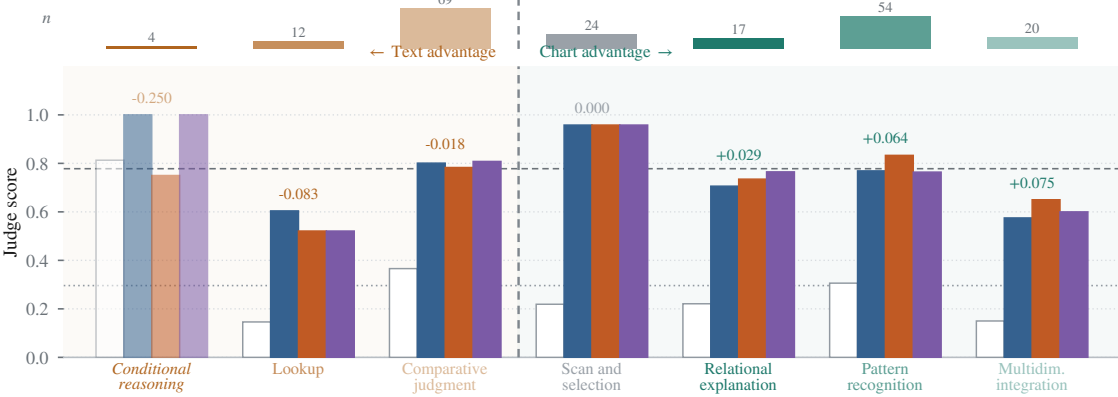
(b) By primary cognitive load
