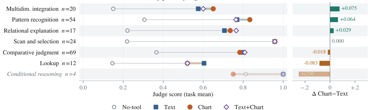
(b) By primary cognitive load
