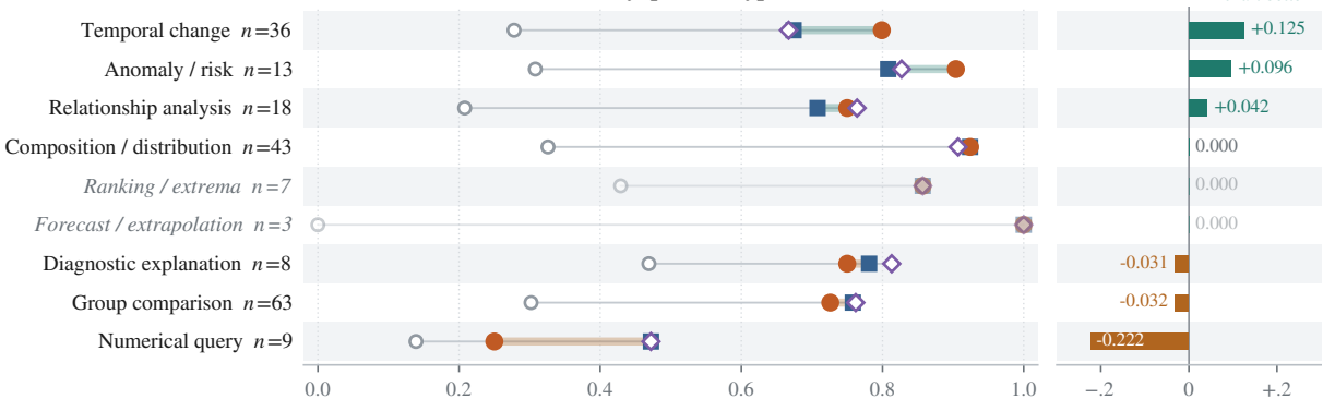
(a) By question type
