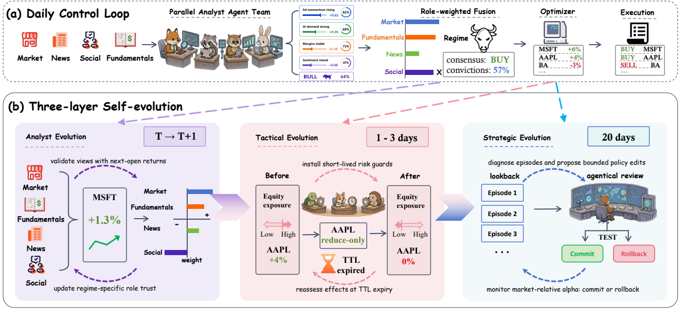
Figure 2: DarwinTrade architecture. The daily control loop (top) maps multi-source evidence to role-weighted signals, constrained portfolio weights, and orders, while delayed realized outcomes (bottom) drive self-evolution of analyst reliability, short-lived tactical guards, and strategic allocator policy through three independently logged loops.
