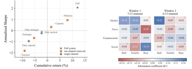
(a) Factorial variants in return–Sharpe space. (b) Regime-conditioned analyst selectivity.
