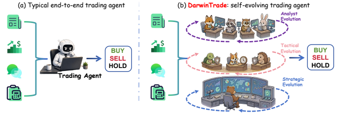
Figure 1: DarwinTrade separates analyst reliability, short-lived tactical guards, and validated allocator changes as three state-disjoint self-evolution loops over a deterministic allocator that the LLM never edits.
