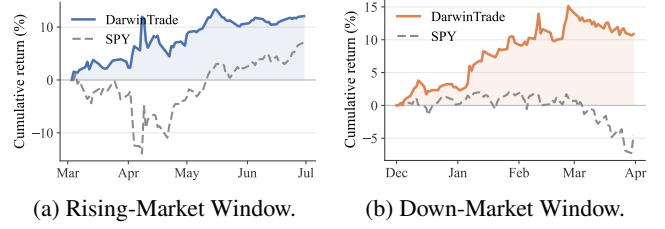
Figure 3: DarwinTrade outperforms SPY in both the Rising-Market and Down-Market Windows under the common 20-stock universe and transaction-cost model, achieving positive cumulative return in a −4.6% down window without re-tuning the controller code or policy space.
