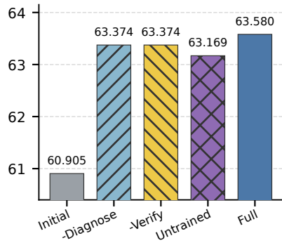
MATH
