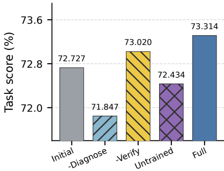
MBPP
