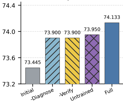
HotpotQA
