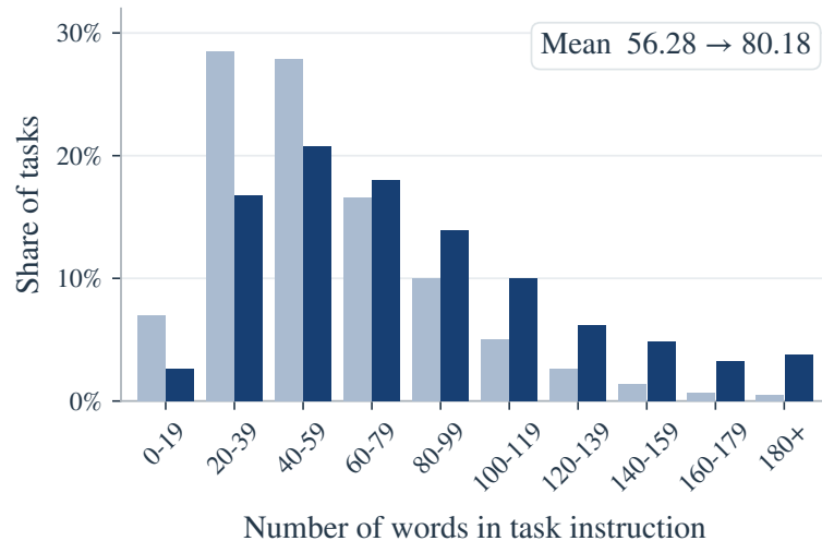
(b) Instruction length
