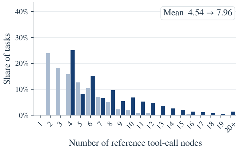
(a) Reference DAG size
