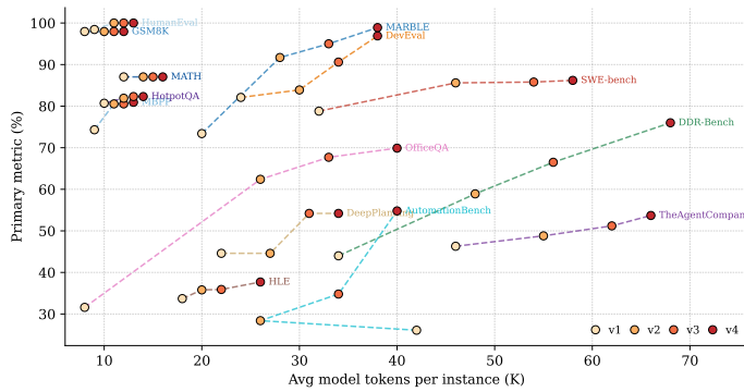
Figure 8: Primary metric against average tokens per instance across the four evolution rounds, with markers running from v_1 to v_4 in increasing darkness. The view separates the accuracy gain from the compute cost of new roles and retry edges.
