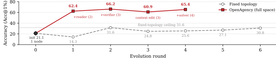
Figure 6: Evolution on OfficeQA Pro under a fixed collaboration graph against evolution over the full space, from one initialization and scored on the same 133 tasks. The fixed arm edits only the shared context, while the full arm may also edit the topology.
