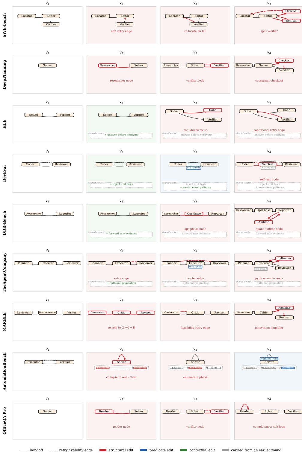
Figure 7: Protocol evolution across rounds on the nine long-horizon and production-oriented benchmarks, which form the rows. Solid ovals are agent roles, small pills inside a dashed container are internal phases of a single-agent solver, solid edges are admissible handoffs, and dashed edges are validity or retry edges. A panel shows everything the protocol carries at that round, where boxed text pinned to an element is a transition or completion predicate and the lower container holds the shared rule and culture. Elements introduced by the current round are drawn in the color of their edit level from Section 3.3, and elements carried from an earlier round are drawn in gray, so a round that leaves the graph unchanged still shows what it revised.
