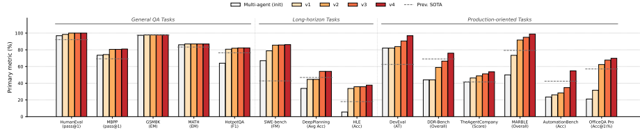
Figure 2: Round-wise trajectory of the primary metric from the initialization v_0 through the evolved rounds v_1-v_4 . Grey dashed lines mark each benchmark’s prior reference.
