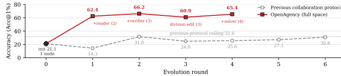
Figure 5: Evolution on OfficeQA Pro from one initialization, scored on the same 133 tasks. The previous-protocol arm edits only the functional division, while the full arm may also change the agent count and the topology.
