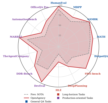
Figure 2: OpenAgency against each benchmark’s prior reference across three categories. The same protocol runs on all fourteen benchmarks.
