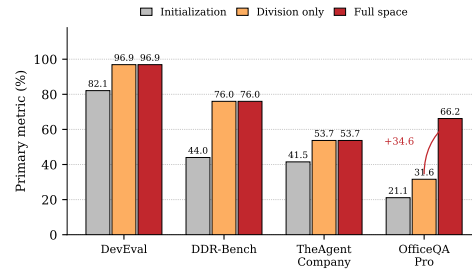
Figure 4: Restricting the evolving space to the functional division against the full space. The restricted arm freezes |\mathcal{N}| and (\mathcal{H}, \mu) at the initialization. Both OfficeQA Pro arms are scored on the same 133 tasks.
