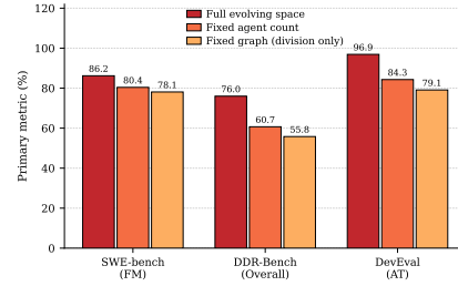
Figure 4: Effect of three evolving spaces. The fixed-count setting holds the agent number, and the division-only setting freezes the whole graph.
