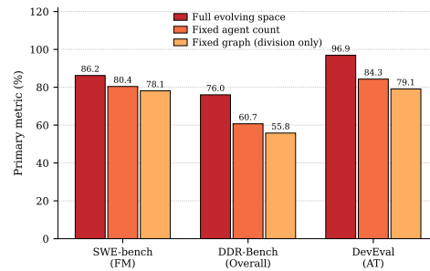
Figure 4: Three nested evolving spaces under one initialization and one evolution loop. The fixed-count arm holds the number of agents |\mathcal{N}| at the initialization, and the division-only arm freezes the whole graph and edits only the functional division.
