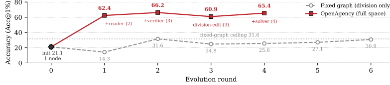
Figure 5: Evolution on OfficeQA Pro under a fixed collaboration graph against evolution over the full space, from one initialization and scored on the same 133 tasks. The fixed arm edits only the functional division, while the full arm may also change the number of agents and the topology.
