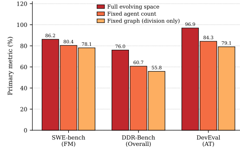
Figure 3: Three nested evolving spaces under one initialization and one evolution loop. The fixed-count arm holds the number of agents |\mathcal{N}| , and the division-only arm freezes the whole graph and edits only the functional division.
