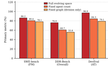
Figure 4: Effect of three evolving spaces. The fixed-count holds the agent number, and the division-only arm freezes the whole graph.
