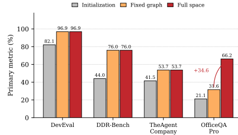
Figure 4: A fixed collaboration graph against the full evolving space. The fixed-graph arm freezes |\mathcal{N}| and (\mathcal{H}, \mu) at the initialization and edits only the functional division. Both OfficeQA Pro arms are scored on the same 133 tasks.
