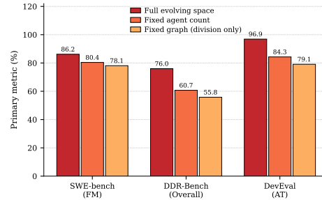
Figure 4: Three nested evolving spaces under one initialization. The fixed-count arm holds the agent count |\mathcal{N}| , and the division-only arm freezes the whole graph.
