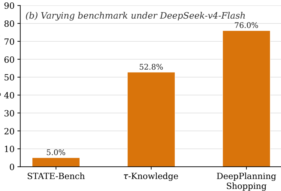
Functional Loop rate in failed trajectories (%)
