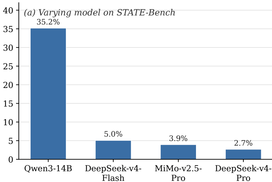
Functional Loop rate in failed trajectories (%)
