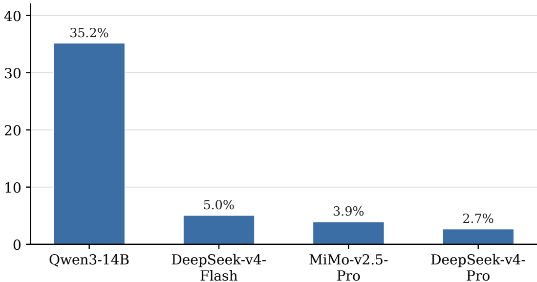
Functional Loop rate in failed trajectories (%)
