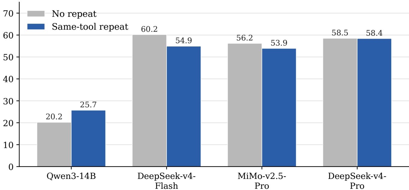
STATE-Bench score (%)
