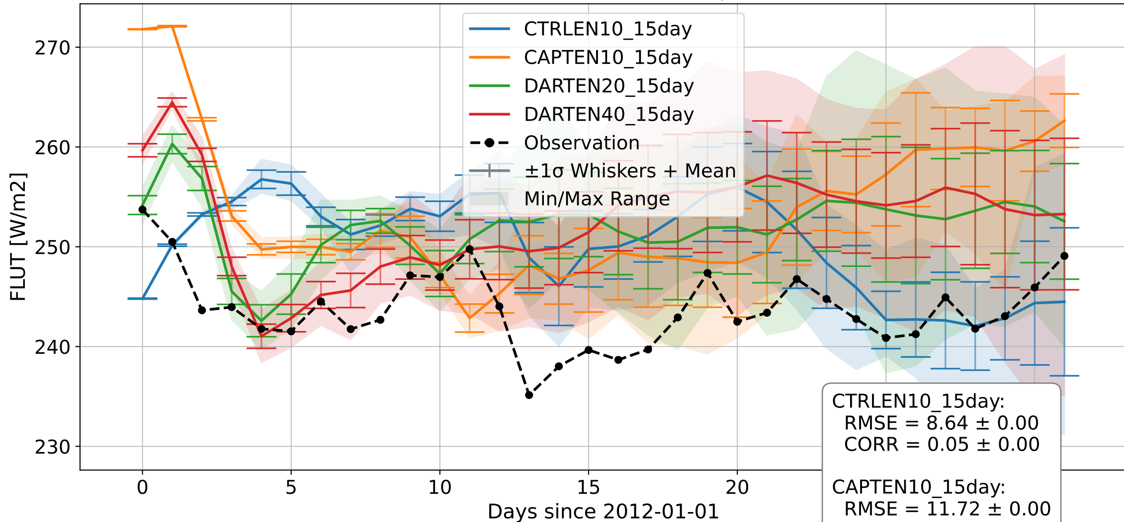
FLUT Time Series over Tropics
