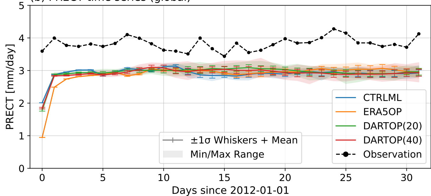
(b) PRECT time series (global)
