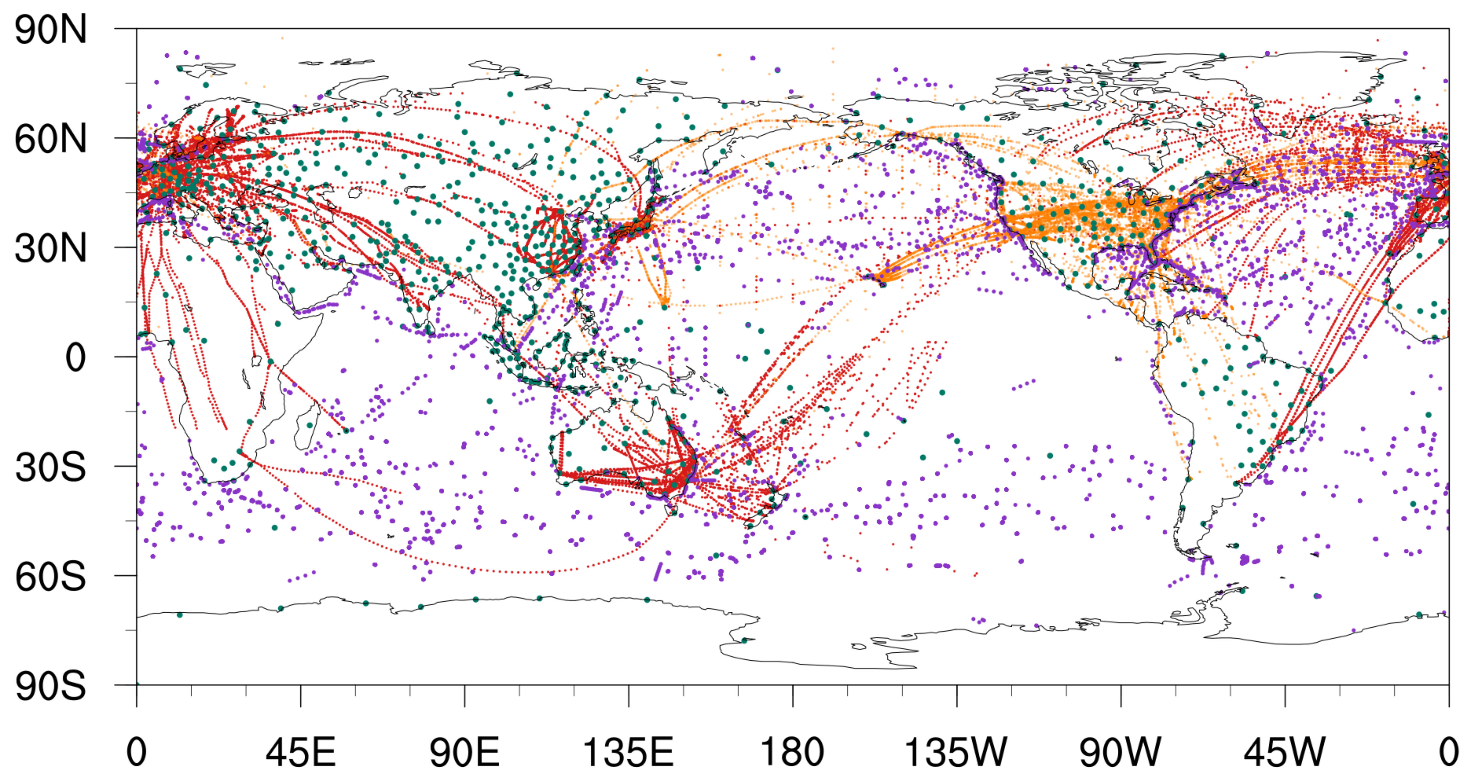
(a) Conventional observations
