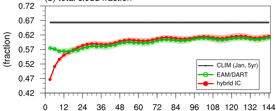
(b) total cloud fraction
