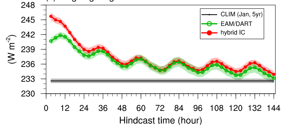
(c) outgoing longwave radiation
