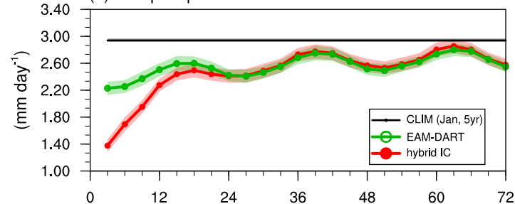
(a) total precipitation
