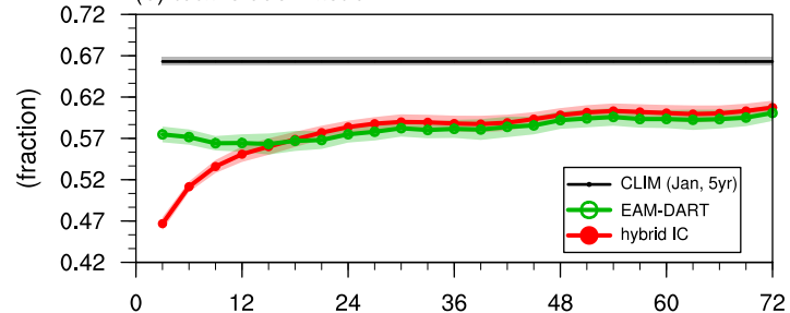
(b) total cloud fraction
