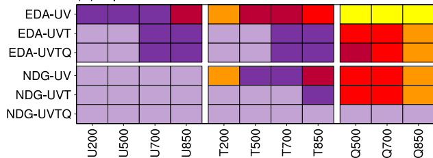
(c) Spatial correlation, mid-latitudes
