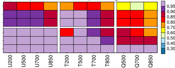
(b) Temporal correlation, polar regions
