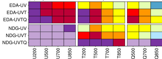
(e) Spatial correlation, tropics
