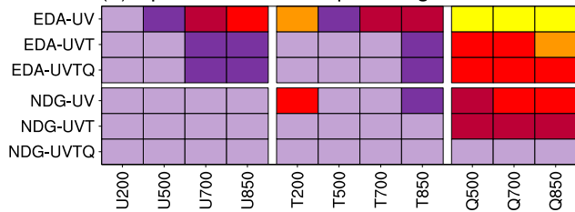
(a) Spatial correlation, polar regions
