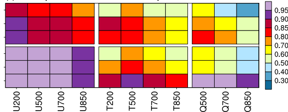
(f) Temporal correlation, tropics
