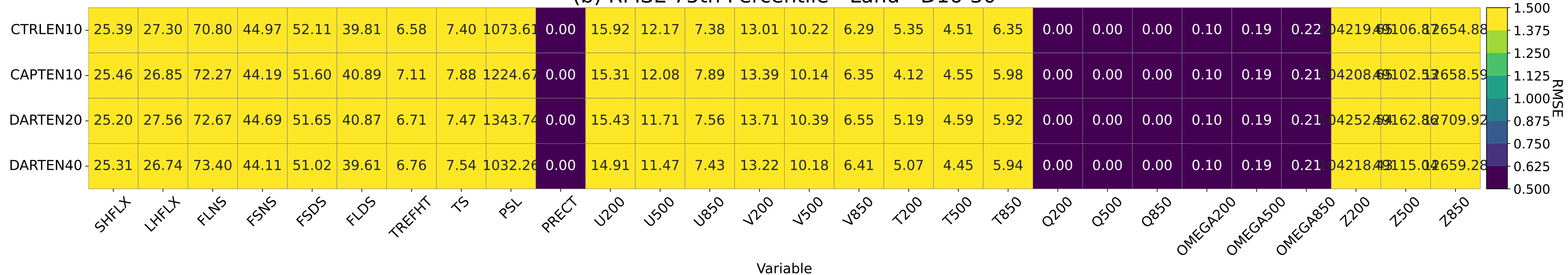
(b) RMSE 75th Percentile - Land - D16-30
