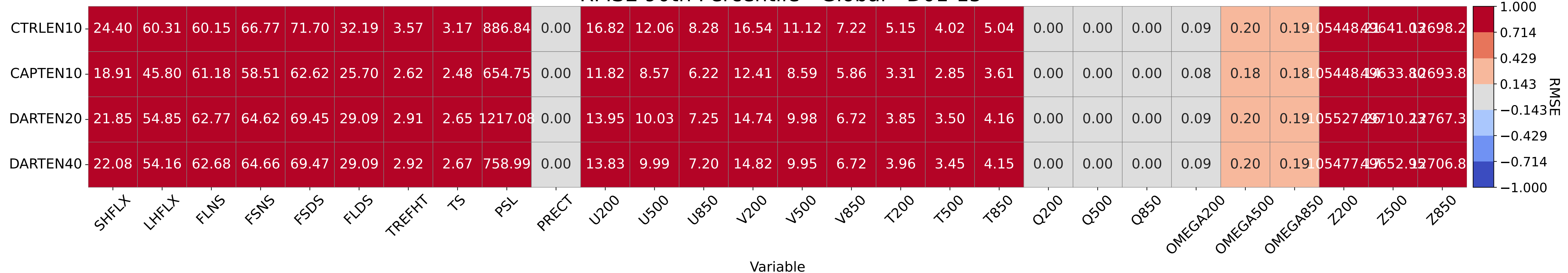
RMSE 90th Percentile - Global - D01-15
