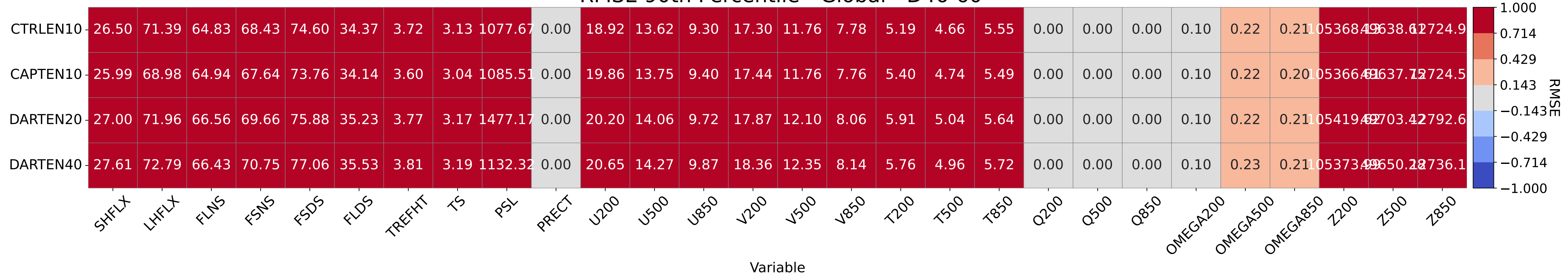
RMSE 90th Percentile - Global - D46-60
