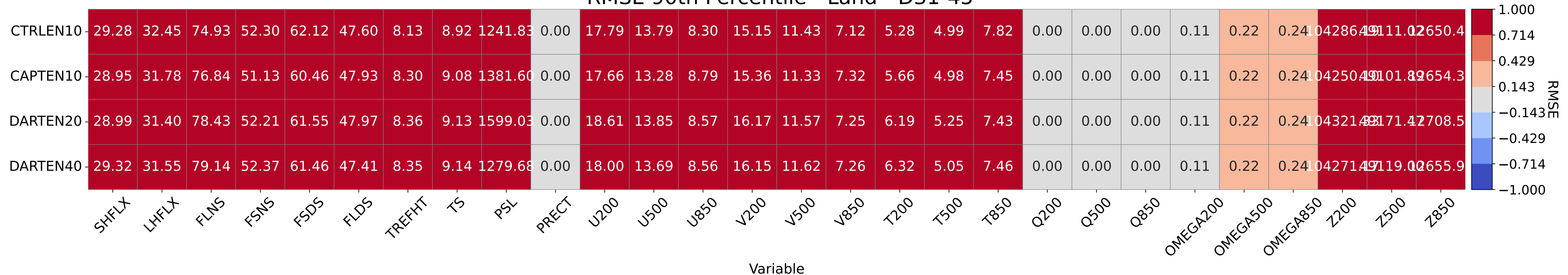
RMSE 90th Percentile - Land - D31-45
