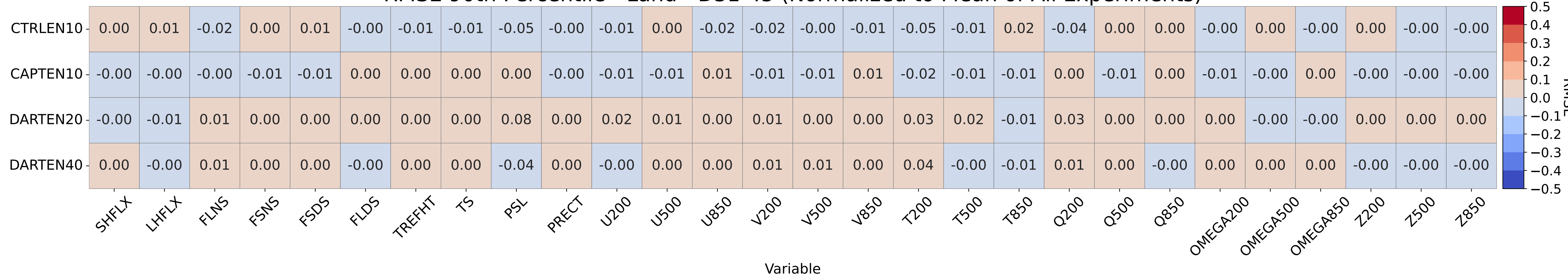
RMSE 90th Percentile - Land - D31-45 (Normalized to Mean of All Experiments)
