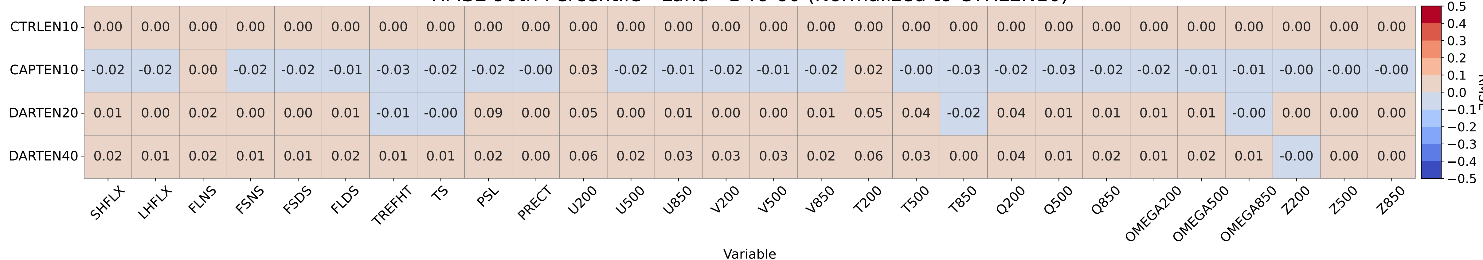
RMSE 90th Percentile - Land - D46-60 (Normalized to CTRLLEN10)
