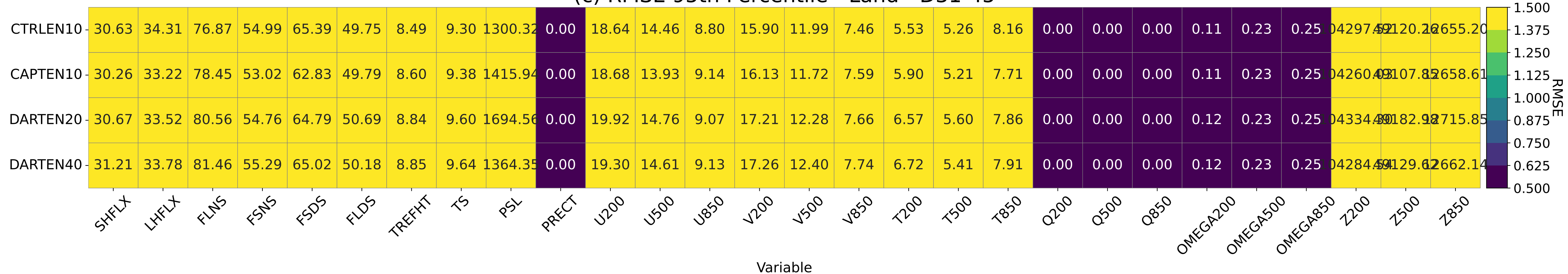
(c) RMSE 95th Percentile - Land - D31-45
