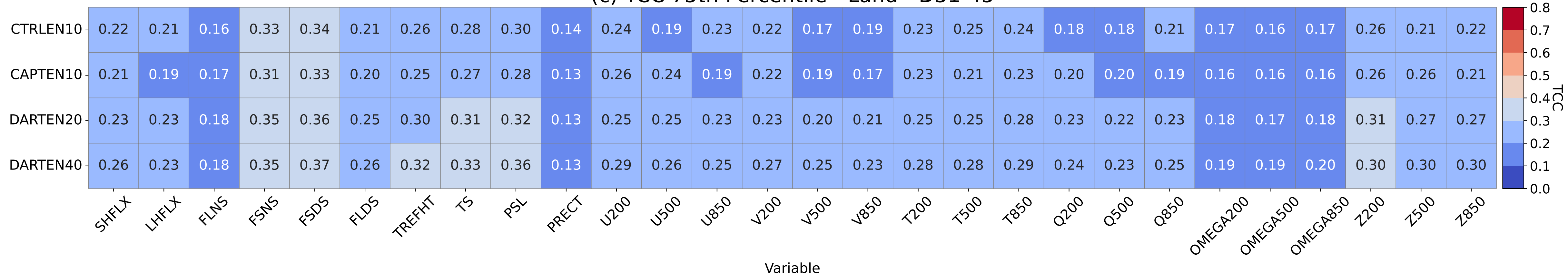
(c) TCC 75th Percentile - Land - D31-45
