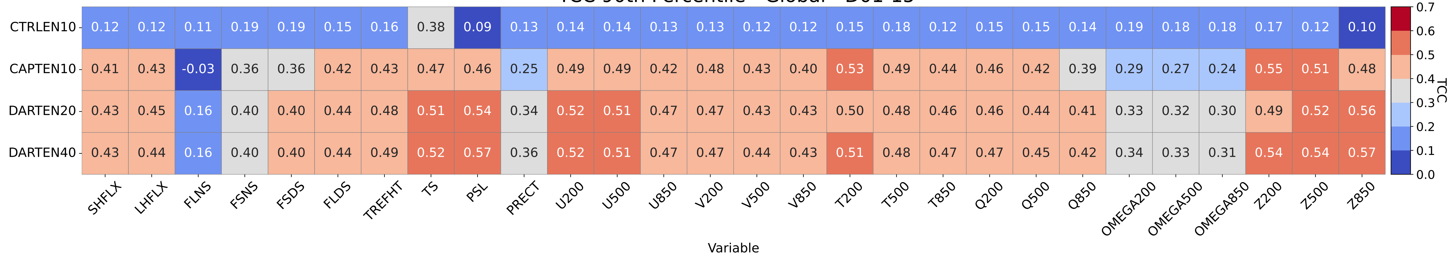
TCC 90th Percentile - Global - D01-15
