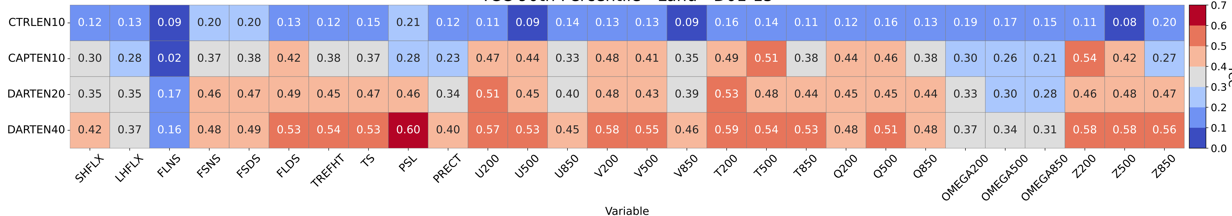
TCC 90th Percentile - Land - D01-15
