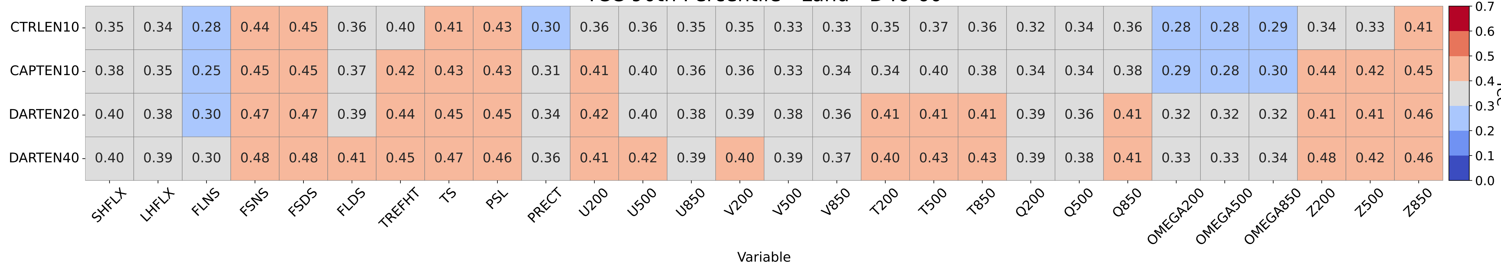
TCC 90th Percentile - Land - D46-60
