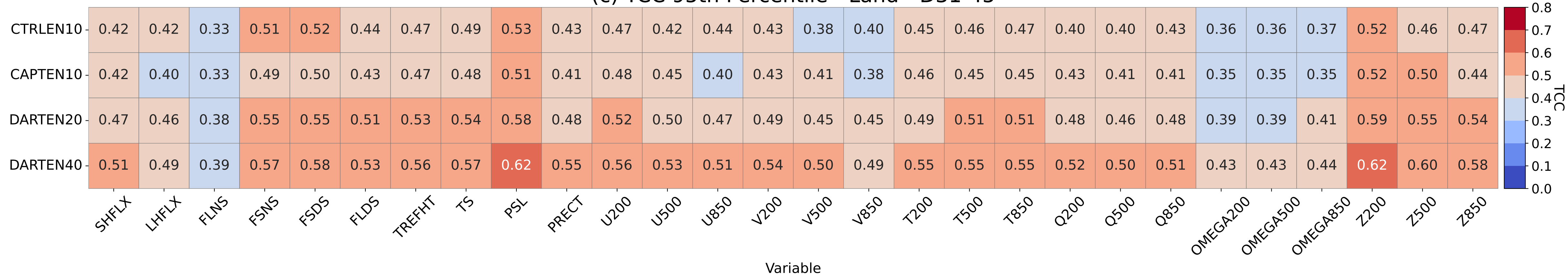
(c) TCC 95th Percentile - Land - D31-45
