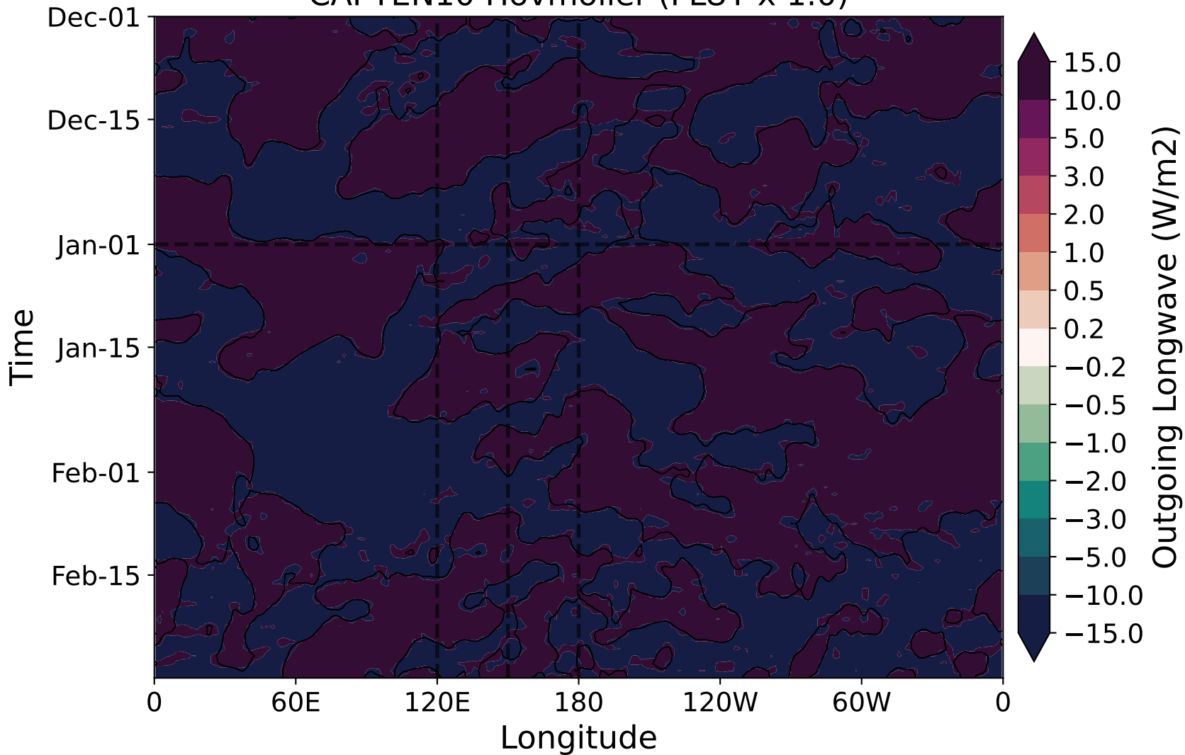
CAPTEN10 Hovmoller (FLUT x 1.0)
